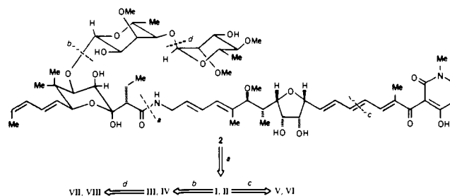
Scheme I. Strategic Bond Disconnections of Aurodox and Efrotomycin a
